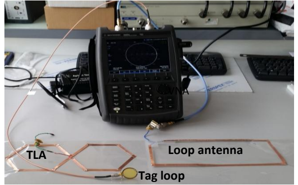
Fig.6 Experiment setup
