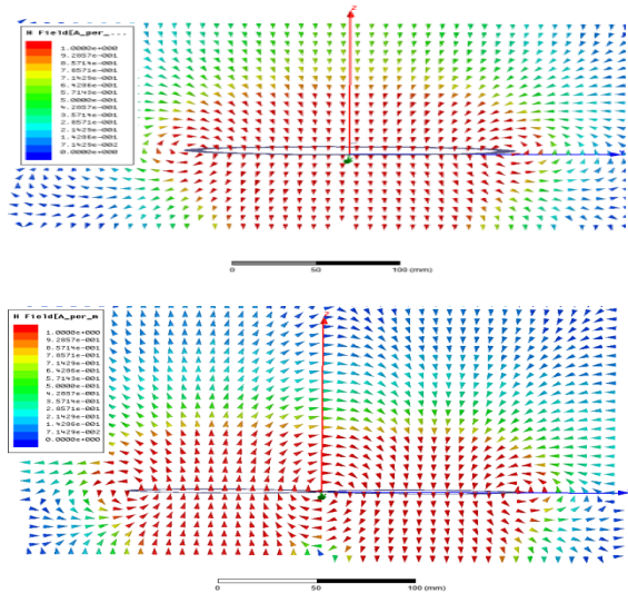
Fig.2.b.Magnetic field distribution for classical loop antenna (top) and TLA (bottom) for a scale of 0 to 1 A/m
