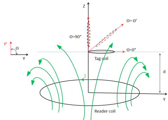
Fig.1: Different positioning of a RFID tag
