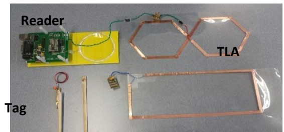
Fig 9. Experimental setup for RFID detection tests
