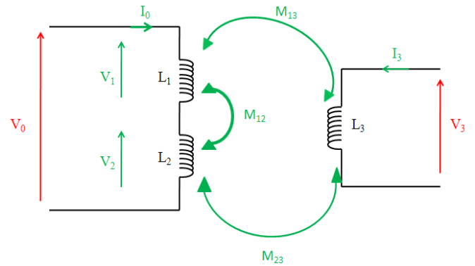
Fig.3. Electrical model for the TLA (left) and a tag (right)
