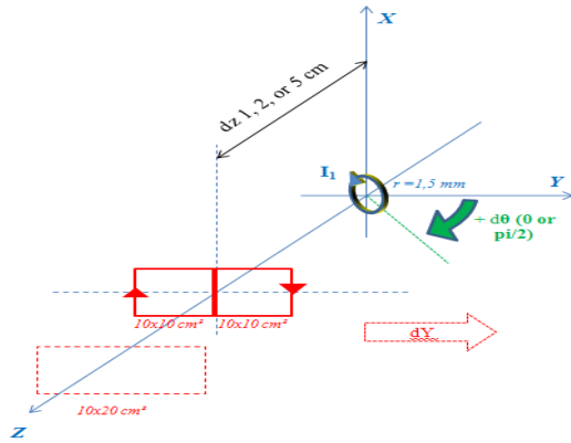
Fig.4. Parametrical studies of the reference loop antenna and TLA
