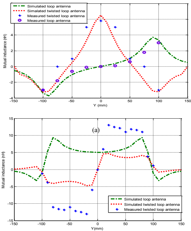
Fig 7. HFSS simulations and measurements for both TLA and rectangular loop antenna in (a) perpendicular and (b) parallel configurations
