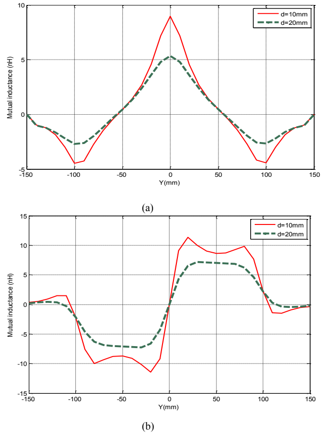
Fig 8 Mutual inductance versus tag-loop distance, (a):perpendicular configuration. (b): parallel configuration (HFSS simulations)
