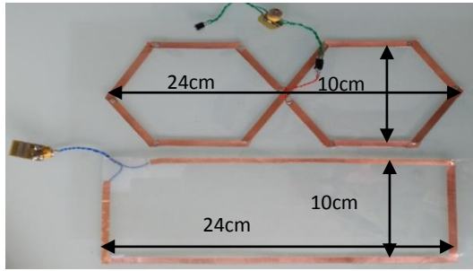
Fig.2a: Loop antenna (bottom) and TLA (top)
