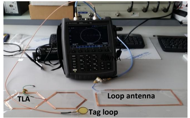
Fig.6 Experiment setup
