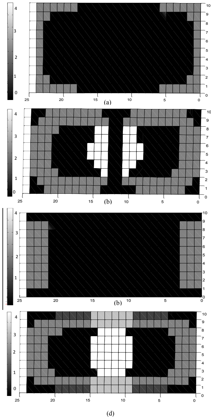
Fig 10. Detection results for: (a): Loop antenna in parallel configuration (b): TLA in parallel configuration (c): Loop antenna in perpendicular configuration (d): TLA in perpendicular configuration
