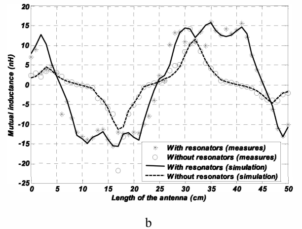
Fig. 5. Equivalent mutual inductance with and without resonators in parallel and perpendicular configuration
