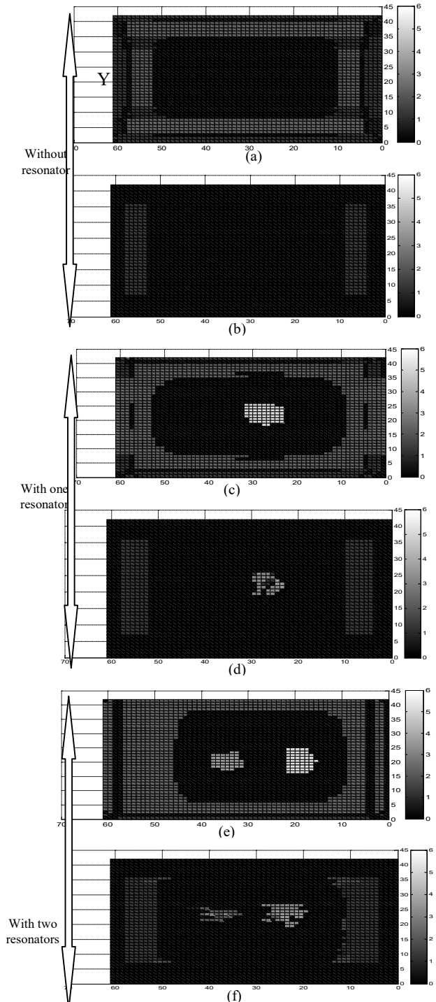
Fig.9 Surface and distance of detection in: Parallel configuration without resonator (a), with one resonator (c), with two resonators (e) and perpendicular configuration without resonator (b), with one resonator (d) with two resonators (f)
