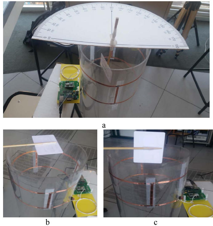
Fig.7. Realized 3D design with the tag inside the tube (a), parallel to the tube (b) and perpendicular to the edges of the tube (c)
