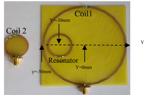
Fig.1. Fabricated tag coil 2 (left) and MCRRC (right)
