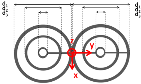
Fig. 1. Layout for 3D fabricated plastic base ( d_1=4.5\text{cm} , d_2=2.5\text{cm} , d_3=0.45\text{cm} )
