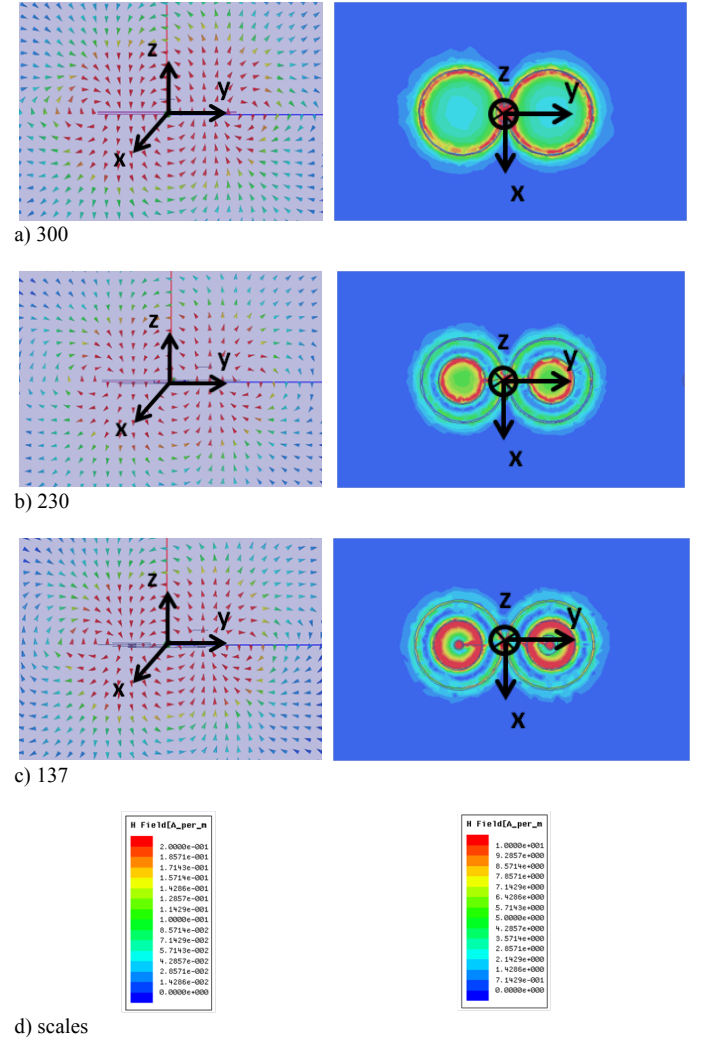
Fig. 2. Displaying of the magnetic field
