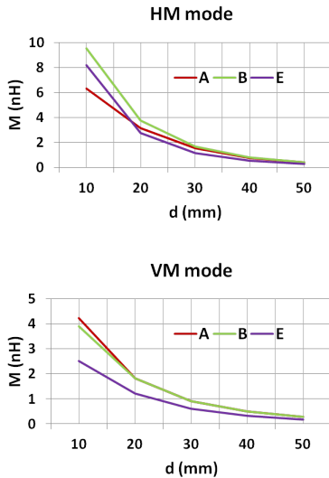
Fig. 6. M versus d (from 10mm to 50 mm by 10mm step) in HM and VM modes
