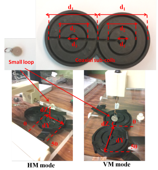
Fig. 3. Experimental setup with DX and DZ variation in millimeter
