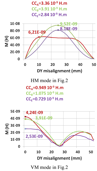
Fig. 4. Simulated mutual inductance M versus lateral misalignment DY at height DZ=10 mm
