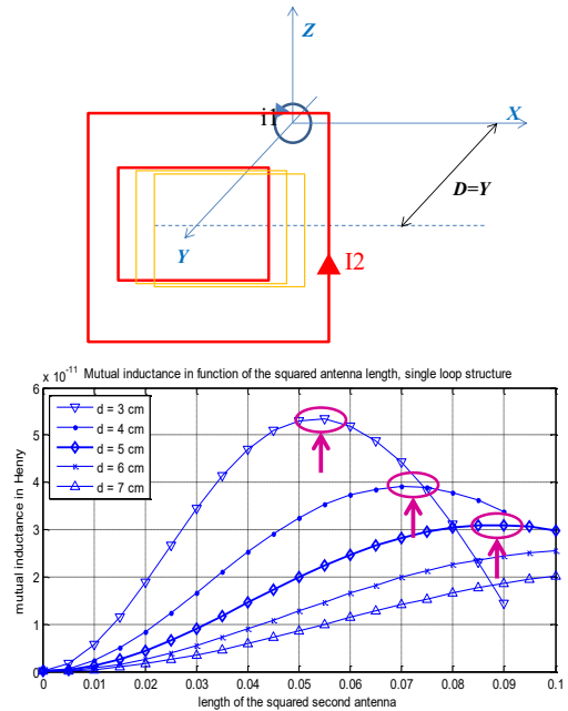
Figure 3 : MATLAB simulation for a single turn coil of 1 cm diameter, in function of the reader loop size at different distance
