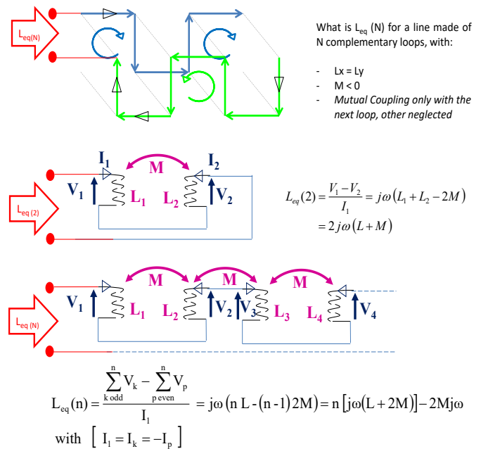
Figure 9 : method for turning a line of “n” complementary loops, and equivalent electrical schematic for determining the inductance value.
