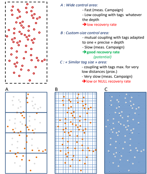
Figure 3 : Equivalent problem of RFID tagged pebbles detection and potential scenarii A, B and C.
