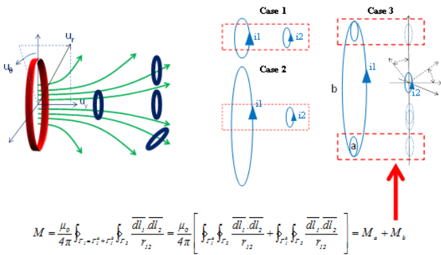
Figure 2 : definition of the Mutual coupling and possible vectorial decomposition of the path in a multi(sub)-loop case
