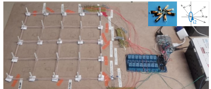
Figure 10 : Prototype of the switched RFID reader loops and lines/columns of complementary sub-loops
