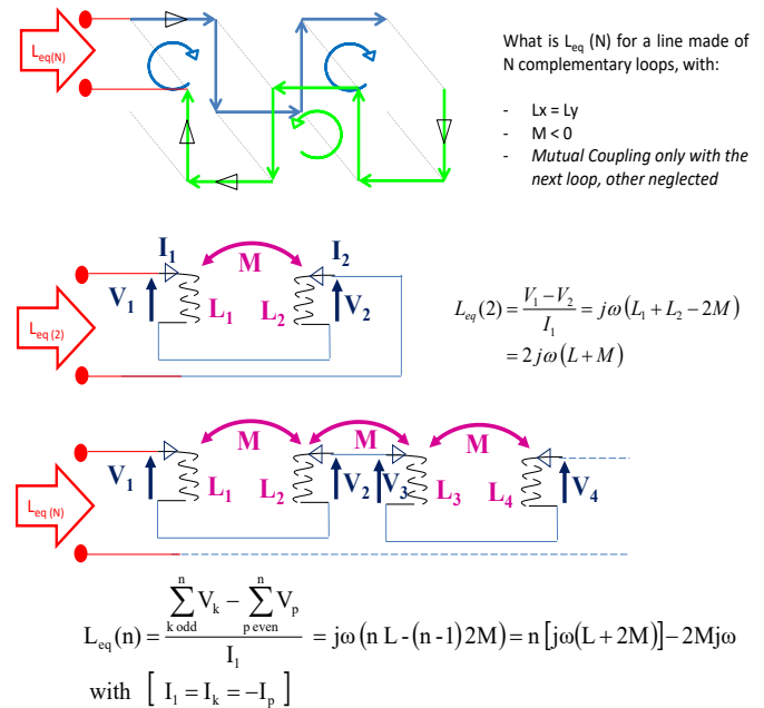
Figure 9 : method for turning a line of “n” complementary loops, and equivalent electrical schematic for determining the inductance value.
