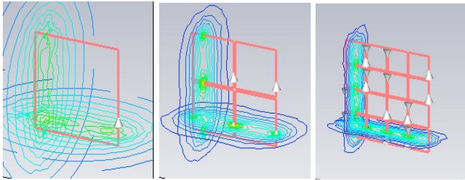
Figure 8 : Magnetic field magnitude, with CST studio, for the single turn 40x40 cm 2 loop, the 4x(20x20) cm 2 C-loop and the 16x(10x10) cm 2 C-loop.
