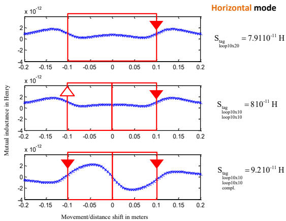
Figure 5 : Mutual induction, in horizontal mode, for the three rectangular loops cases in Figure 4, and evaluation of the S factor.
