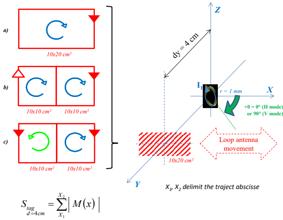
Figure 4 : Simulation of the complementary-loops structure in the case of an equivalent circular surface (radius 1mm) and 3 reader loop cases. Definition of the S factor.
