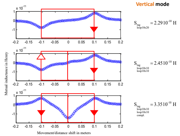
Figure 6 : Mutual induction, in vertical mode, for the three rectangular loops cases in Figure 4, and evaluation of the S factor.
