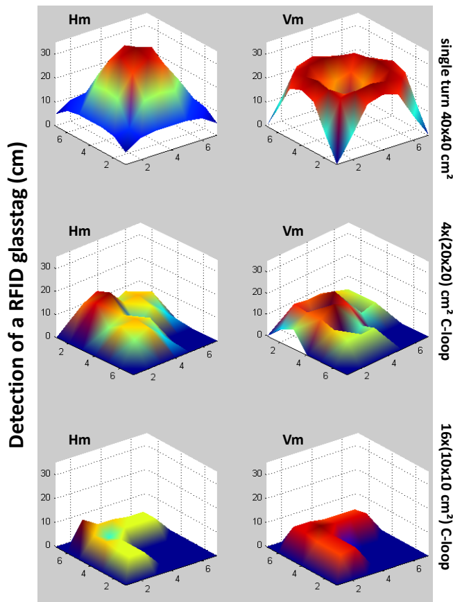
Figure 11 : Detection performances, in cm, of a RFID glasstag in horizontal (left) and vertical (right) mode, for the three structures: the single turn 40x40 cm 2 loop (top), the 4x(20x20) cm 2 C-loop (middle) and the 16x(10x10) cm 2 C-loop (bottom)
