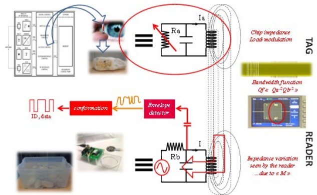
Figure 1 : Principle of pebble tagged in RFID with LF glasstag.
