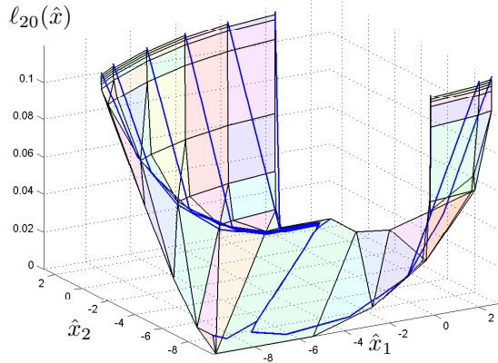
Fig. 2. The constructed convex lifting \ell_{20}(\hat{x}) over \mathcal{K}_{20}(\Omega_{\hat{x}}) with h_1 = 10^{-2} and \epsilon = 10^{-3} and its strict decrease along the closed-loop dynamics of the observer system (3) outside \Omega_{\hat{x}} .
