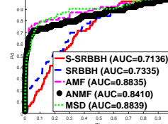
Fig. 5. ROC: Case 2
