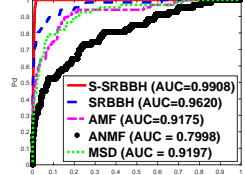
Fig. 11. ROC: Case 3
