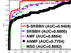
Fig. 9. ROC: Case 1
