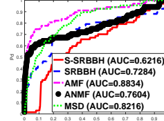
Fig. 10. ROC: Case 2
