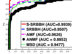
Fig. 4. ROC: Case 1
