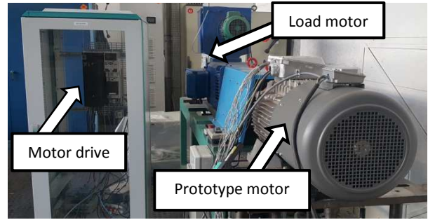
Fig.21 Experimental setup
