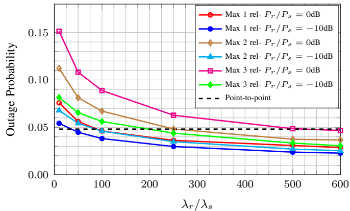
Fig. 3. Outage probability for NNC as a function of the relative density between relays and sources, for different relay-source relative transmission powers. \lambda_s = 10^{-4} , R = 1\text{b/use} , \alpha = 4 . Relays are chosen centered around the destination ( \epsilon = 1 ). OP is optimized w.r.t. the noise compression variance.
