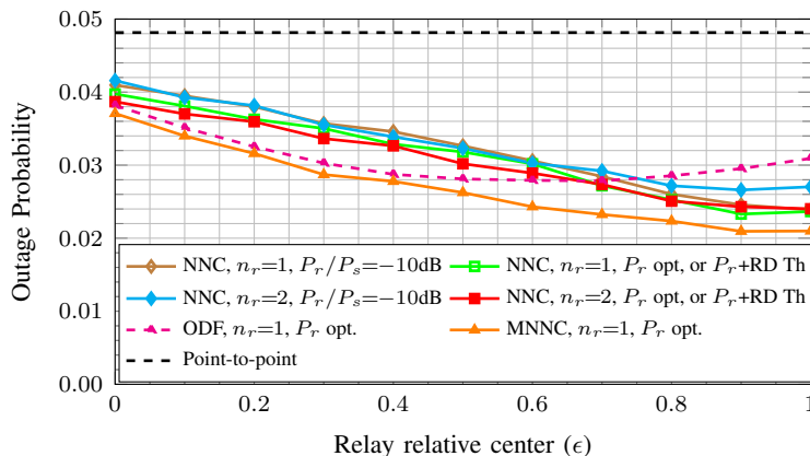
Fig. 14. Outage probability for NNC with optimized relay power and thresholds, compared to the best performance obtained with MNNC and ODF. \lambda_r/\lambda_s = 500 , \lambda_s = 10^{-4} , R = 1\text{b/use} , \alpha = 4 . OP is optimized w.r.t. the noise compression variance.
