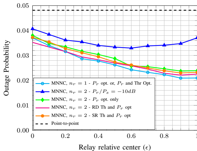
Fig. 11. Outage probability for MNNC with optimized relay power and thresholds. \lambda_r/\lambda_s = 500 , \lambda_s = 10^{-4} , R = 1\text{b/use} , \alpha = 4 .
