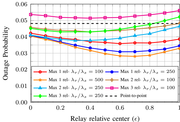
Fig. 8. Outage probability for ODF as a function point around which the relays are chosen, one the line between source and destination, for different relative densities. P_r/P_s = -10\text{dB} , \lambda_s = 10^{-4} , R = 1\text{b/use} , \alpha = 4 .
