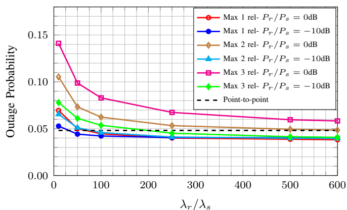
Fig. 2. Outage probability for ODF as a function of the relative density between relays and sources, for different relay-source relative transmission powers. \lambda_s = 10^{-4} , R = 1\text{b/use} , \alpha = 4 . Relays are chosen centered around the source ( \epsilon = 0 ).
