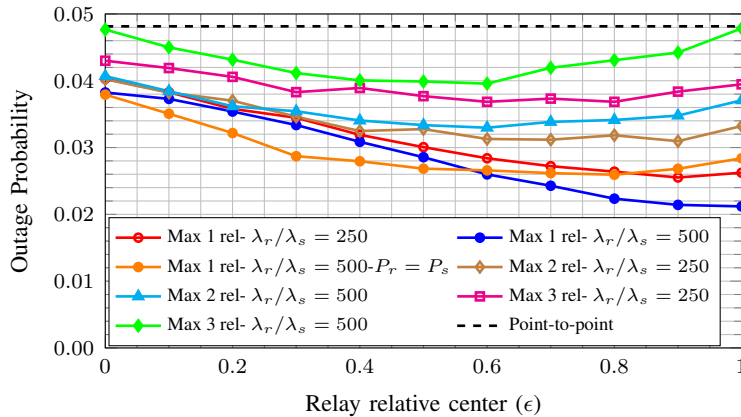
Fig. 10. Outage probability for MNNC as a function point around which the relays are chosen, one the line between source and destination, for different relative densities. P_r/P_s = -10\text{dB} , \lambda_s = 10^{-4} , R = 1\text{b/use} , \alpha = 4 . OP is optimized w.r.t. the noise compression variance.
