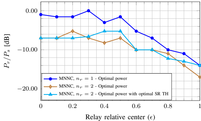
Fig. 12. Optimal power for MNNC corresponding to the OP of Fig. 11. Using more than one relay allows the reduction of the relay power. \lambda_r/\lambda_s = 500 , \lambda_s = 10^{-4} , R = 1\text{b/use} , \alpha = 4 .
