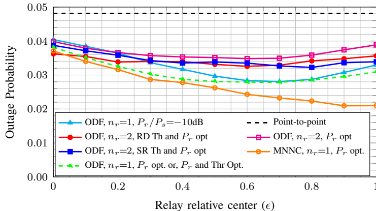
Fig. 13. Outage probability for ODF with optimized relay power and thresholds, compared to the best performance obtained with MNNC. \lambda_r/\lambda_s = 500 , \lambda_s = 10^{-4} , R = 1\text{b/use} , \alpha = 4 .
