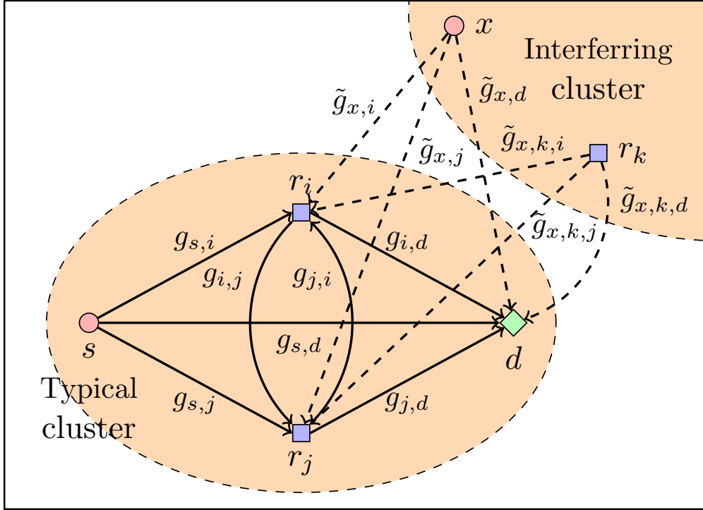
Fig. 1. Representation of the network and relevant channel involved. d denotes the typical destination at origin, and s is the typical source at p_s = (-D, 0) .
