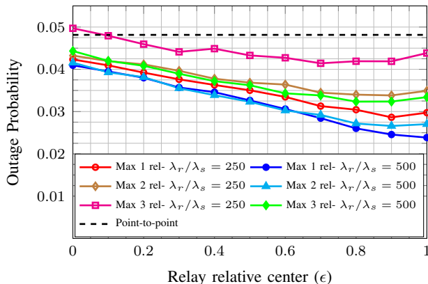
Fig. 9. Outage probability for NNC as a function point around which the relays are chosen, one the line between source and destination, for different relative densities. P_r/P_s = -10\text{dB} , \lambda_s = 10^{-4} , R = 1\text{b/use} , \alpha = 4 . d = 10 . OP is optimized w.r.t. the noise compression variance.
