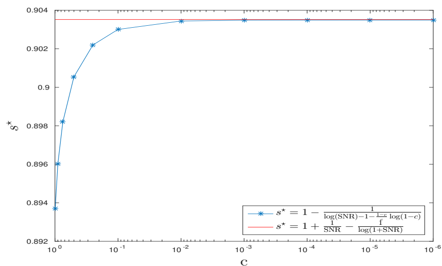
Figure 6. CPD scenario: s^* vs. c , \text{SNR} = 45 dB.
