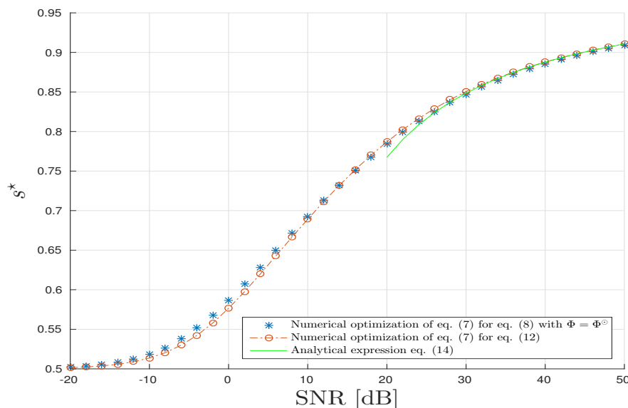
Figure 4. Canonical Polyadic Decomposition (CPD) scenario: Optimal s -parameter versus Signal to Noise Ratio (SNR) in dB.
