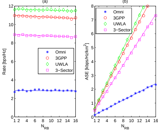
Fig. 4: \mathcal{R}/\ln(2) (a) and ASE (b). Markers: Monte Carlo simulations. Solid lines: IM-based approximation (three-ball). Setup: “Empirical” in Table VIII, R_{MT} = 7.6 m.
