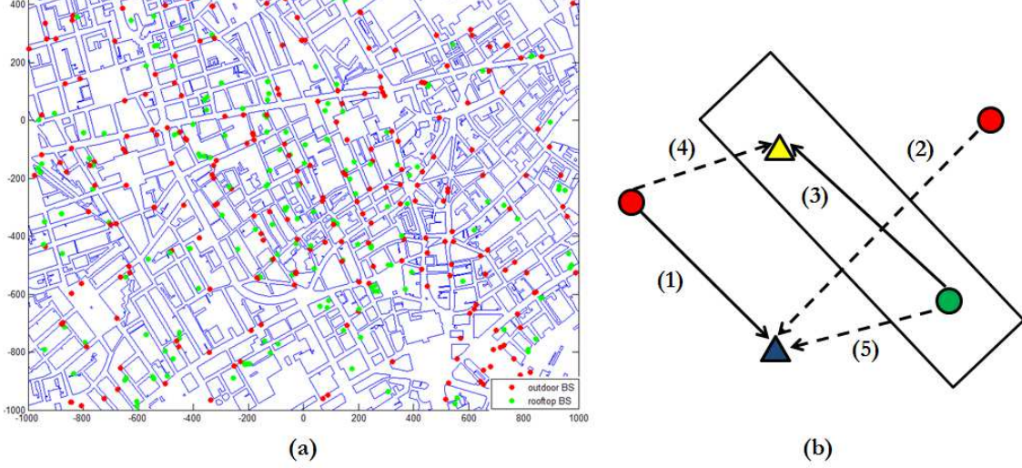
Fig. 1: Considered cellular network (a) and multi-state blockage model (b). (a) It is obtained from the dataset in [7] and represents a dense urban environment in downtown London. The red and green dots represent BSs that are located outside and inside the buildings, respectively. The blue shapes represent the buildings in the considered region. (b) It provides a sketched illustration of a multi-state blockage model (dots: BSs, triangles: MTs): (1) outdoor LOS link, (2) outdoor NLOS link, (3) indoor LOS link, (4) outdoor-to-indoor link, (5) indoor-to-outdoor link. Every type of link has a different probability of occurrence and the corresponding channels have different parameters.
