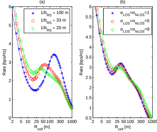
Fig. 8: \mathcal{R}/\ln(2) vs. density of blockages (a) and shadowing severity (b). Markers: Monte Carlo simulations. Solid lines: IM-based approximation (three-ball). Setup: “RS” in Table VIII, PPP-distributed BSs, R_{MT} = 11.9 m, N_{RB} = 1 , Omni antennas.
