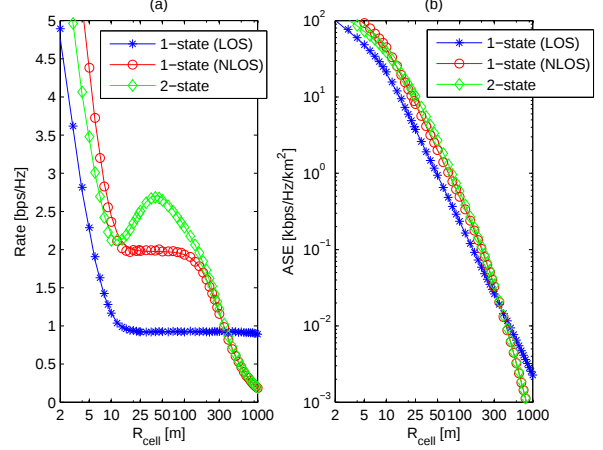
Fig. 3: \mathcal{R}/\ln(2) (a) and ASE (b) of one- and two-state blockage models. Markers: Monte Carlo simulations. Solid lines: IM-based approximation (three-ball). Setup: “RS” in Table VIII, PPP-distributed BSs, N_{RB} = 8 , R_{MT} = 3.9 m, Omni antennas.
