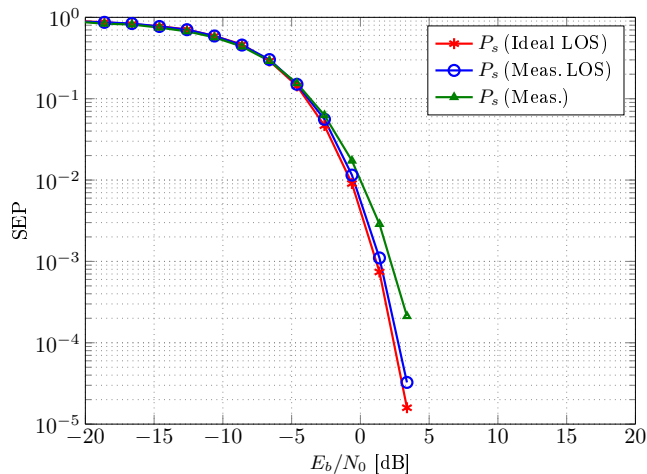
(a) Scenario I, 4 \times 4 MIMO with \eta = 1
