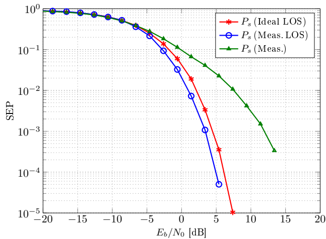
(c) Scenario I, 4 \times 4 MIMO with \eta = 2
