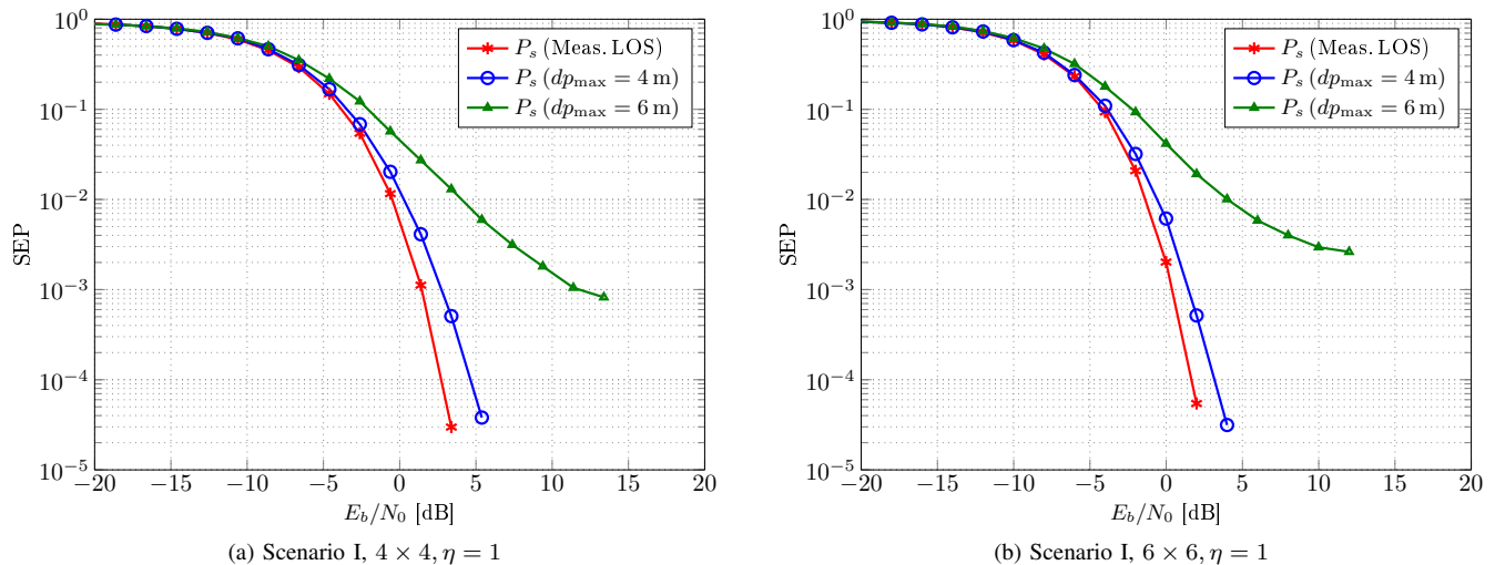
Fig. 12. Simulation results on the SEP of GSM over the measured channels (Scenario I). Legend: “Meas. LOS” — LOS component extracted from the measured multipath channels and using (7); dp_{\max} — measured multipath channels and using the algorithm given in Appendix B-3, but the MIMO CIRs are truncated to include only paths with a path length not exceeding dp_{\max} .
