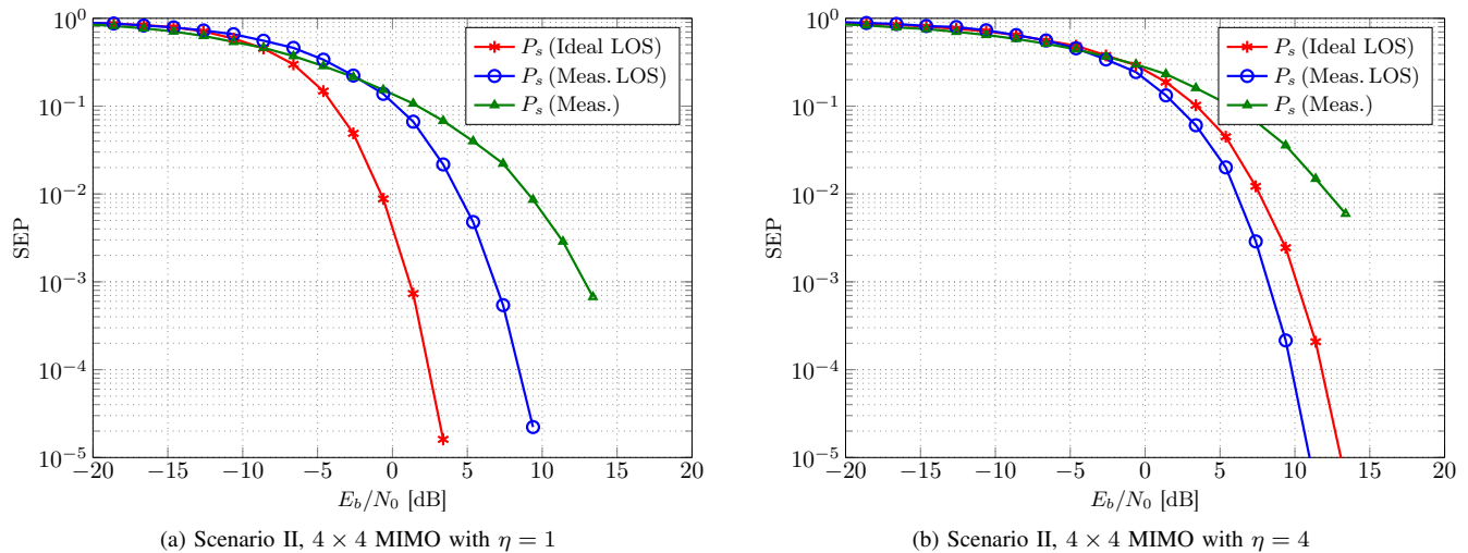
Fig. 13. Simulation results on the SEP of GSM (Scenario II). The legend terms are the same as in Fig. 10.
