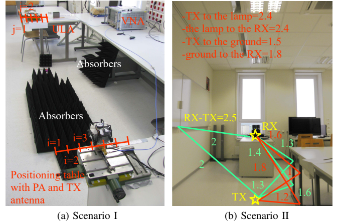
Fig. 4. The measurement site. All dimensions in (b) are in meters.
