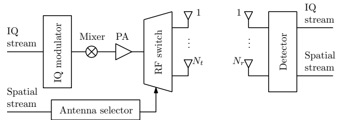
Fig. 1. Conceptual architecture for SM/GSM MIMO.
