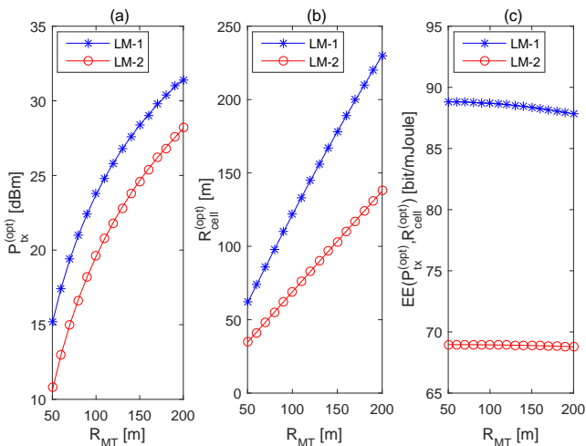
Fig. 7. Optimal transmit power (a), density of BSs ( R_{\text{cell}} ) (b), and energy efficiency (c) versus the density of MTs ( R_{\text{MT}} ). Solid lines: Optimum from the algorithm in Table III. Markers: Optimum from a brute-force search of (21). LM-1: Load Model 1 and LM-2: Load Model 2.
