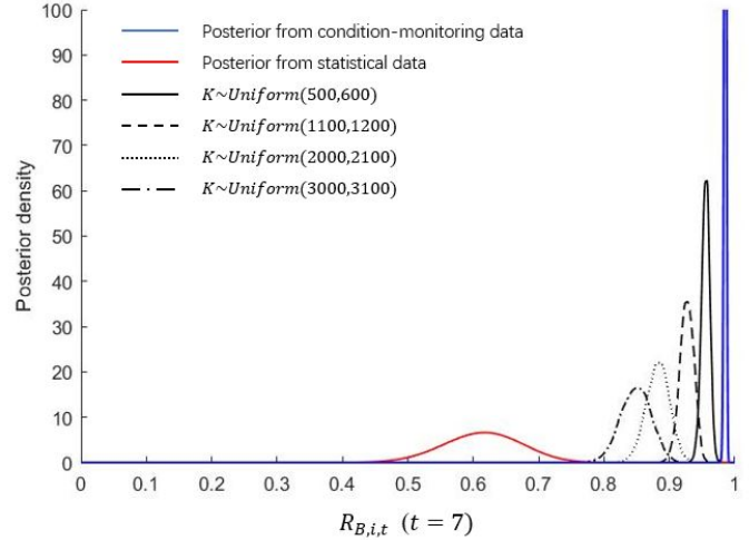
Fig. 7. Posterior distributions under different initial distributions of K
