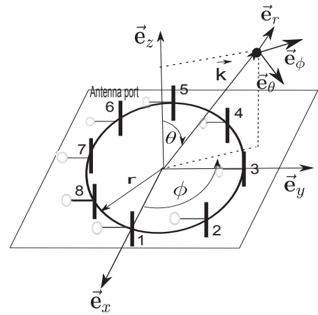
Fig. 1. Antenna configuration.
