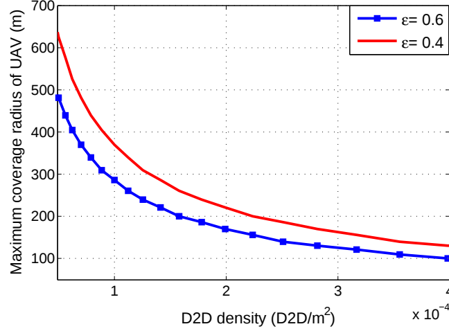
Figure 10: Maximum UAV coverage radius vs. D2D density (number of D2D pairs per \text{m}^2 ).
