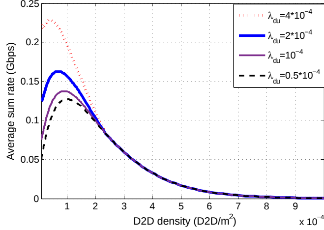
Figure 6: Average sum-rate vs. D2D density (number of D2D pairs per \text{m}^2 ).
