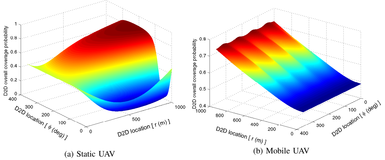
Figure 15: Overall D2D coverage probability vs. location of a D2D user.
