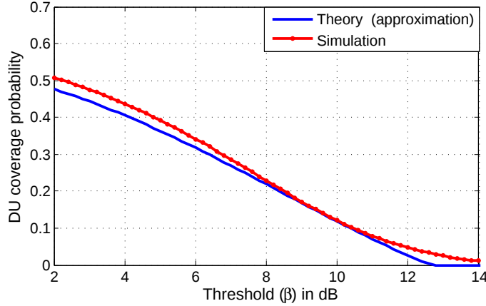
Figure 4: DU coverage probability vs. SINR threshold.
