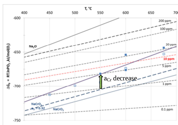
Fig. 7. Oxygen potentials in the Cr-O-Na system as function of temperature for sodium oxide and chromite oxide formation (Free energies of formation for \text{Na}_2\text{O} and \text{NaCrO}_2 from Hsc. 5.11 software, Thorley oxygen solubility relation, experimental observations of sodium chromite on 316L plotted as full square with mean squared fitting [26])
