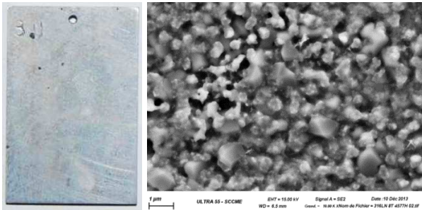
Fig. 3. Photo and SEM surface observation (secondary electrons) of the sample (20x30x1.5 mm) immersed from the beginning of the test for 4600 h at 550 °C in liquid sodium with low oxygen content.
