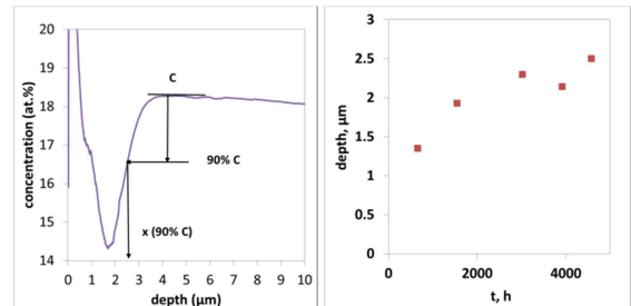
Fig. 5. GD-OES depth 4600 h Cr profile of the Cr depleted zone and method of estimation of the extent of Cr depleted zone (c : Cr concentration of the bulk, x : depth for 90% of c).
