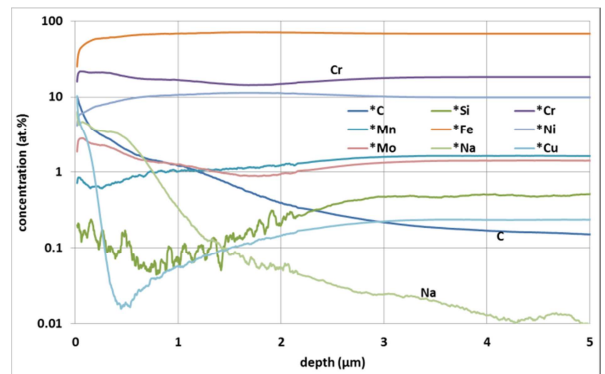
Fig. 4. GD-OES depth chemical profiles in log. scale of the dissolution zone for the sample immersed from the beginning of the test for 4600 h at 550 °C in liquid sodium with low oxygen content.
