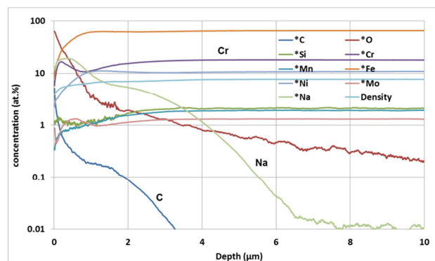
Fig. 2. GD-OES depth chemical profiles in log. scale of the oxide zone for the sample immersed during the last 3900 h (periods 2+3+4+5) of the test at 550 °C in liquid sodium with low oxygen content.
