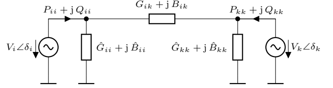
Fig. 1. Single line equivalent circuit for active and reactive power flow.
