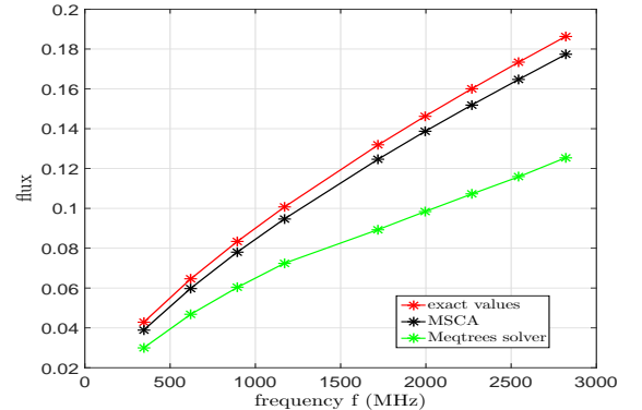
Fig. 3. Recovered flux of one weak outlier source after calibration for F = 9 .
