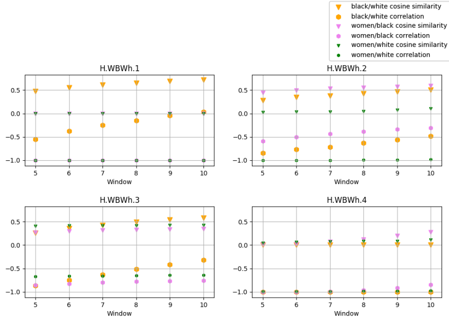
Fig. 1. Hate speeches H.WBWh.1-4. In H.WBWh.1, black and white show a high similarity score though they are not correlated. In the text, the meaning of “white” is modified both by the prefix anti- and by the presence of black .
