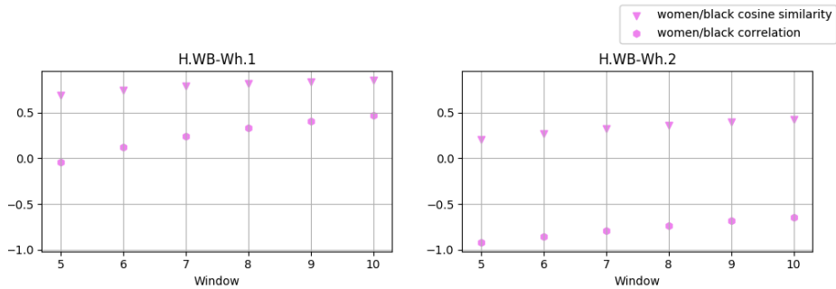
Fig. 5. Hate speeches H.WB-Wh.1-2. H.WB-Wh.1 is about black women , opposed to black men ; H.WB-Wh.2 carries on an analogy between blacks’ rights and women’s rights
