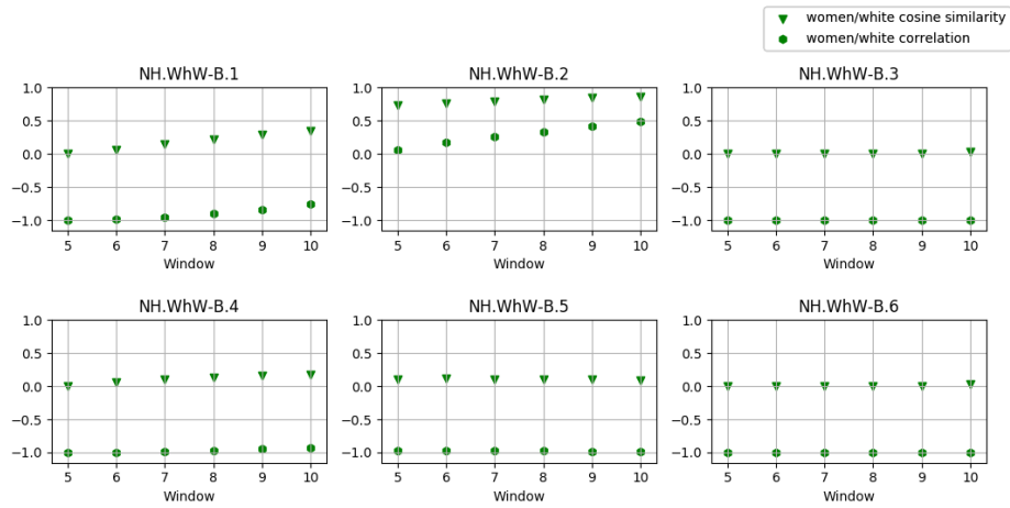
Fig. 4. Non-hate speeches NH.WhW-B.1-6. Five out of six documents show a maximal anticorrelation and a 0 similarity (“Ivanka Voters”). NH.WhW-B.2 is about white women (“Ivanka Voters”).
