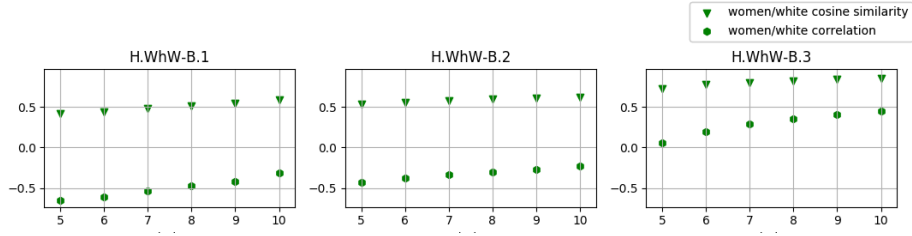
Fig. 3. Hate speeches H.WhW-B.1-3. In particular, in H.WhW-B.1-2 the keywords occur without a strong relation, whereas H.WhW-B.3 is explicitly on white women
