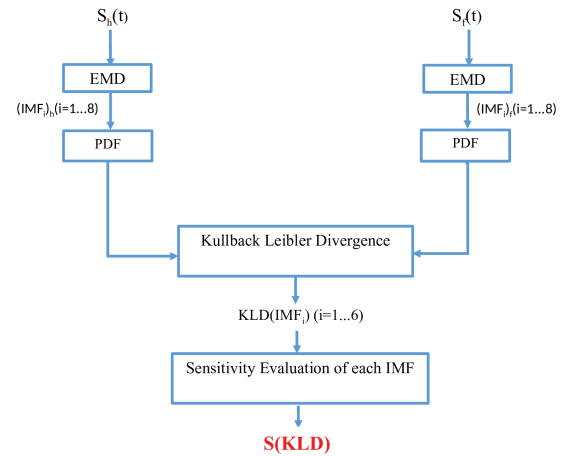
Fig. 6. Flowchart of the KLD sensitivity evolution
