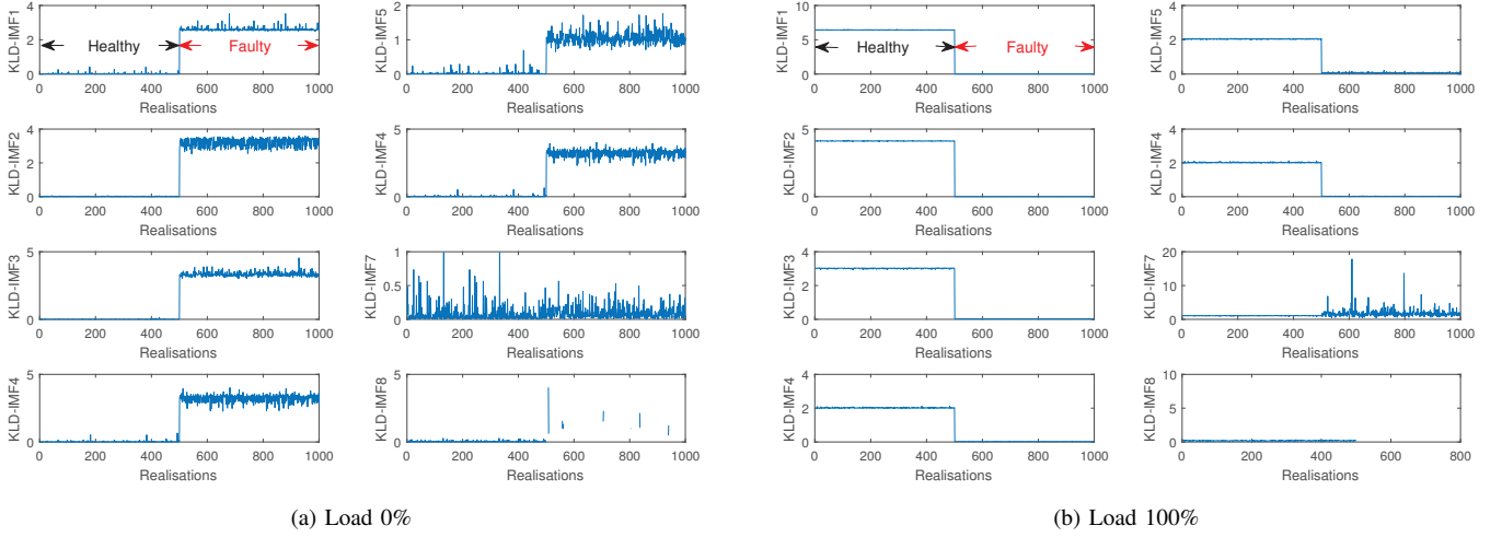
Fig. 5. KLD evolution for each retained IMF
