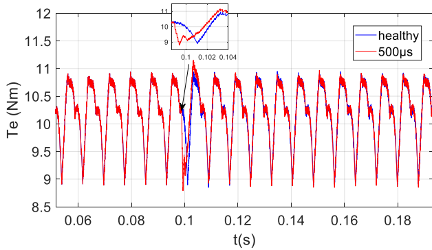
Fig. 1. Intermittent 500 \mu s fault impact on current and torque
