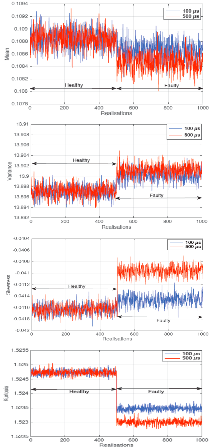
Fig. 4. Statistical moments for the two faults with SNR= 40dB
