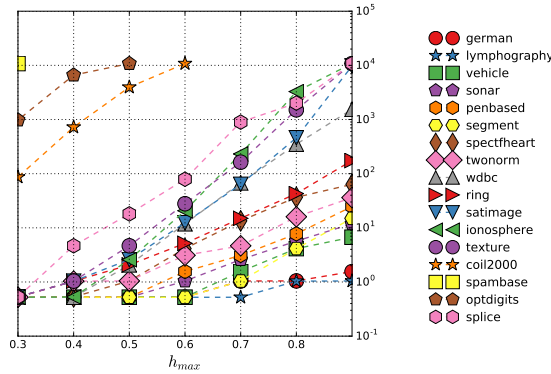
Fig. 4. HFP-growth’s processing times (in seconds)
