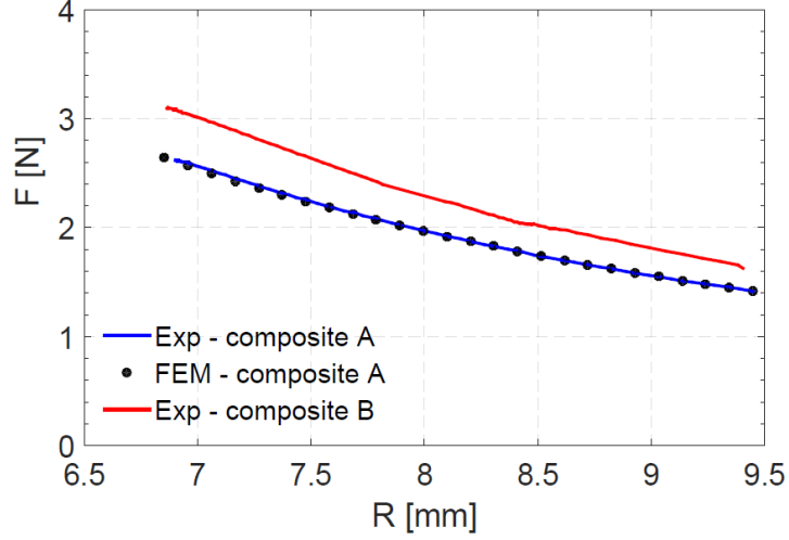
Figure 7: Comparison of the reaction force from composite simulation to experimental measurements
