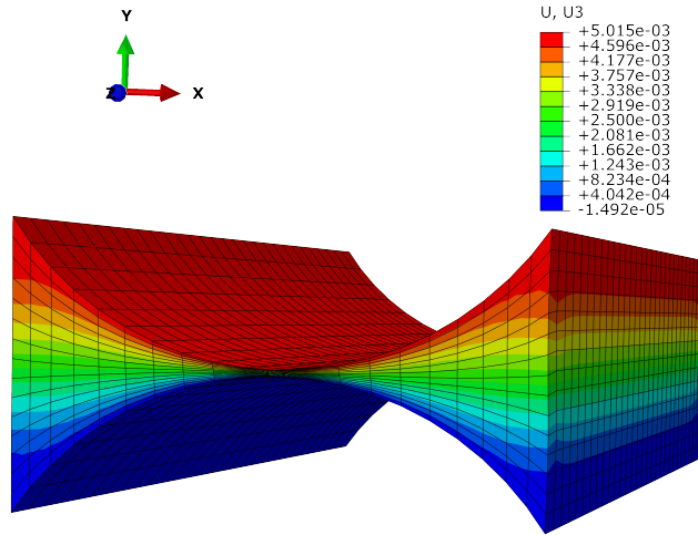
Figure 10: Shearing of the matrix between 2 wires
