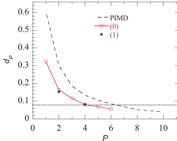
Figure 6: Divergence factor, d_P , (generalisation of eq 29 in 3D) as a function of the number of beads for the proton distribution in BZO at T = 300 K obtained by PIMD and QTB-PIMD simulations using either f_P^{(0)} or f_P^{(1)} , herein referenced as (0) and (1), respectively. The horizontal dotted line allows one to determine the number of beads corresponding to d_P = 0.08 .
