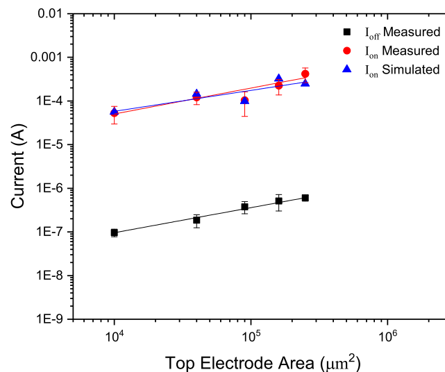
FIG. 5. Dependence of current on top electrode area of Au/ \text{Li}_x\text{CoO}_2 /SiO 2 /Si memristive cells: experimental I_{\text{off}} (at -2 V; black squares), experimental I_{\text{on}} (at -2 V; red circles) and simulated I_{\text{on}} (at -2 V; blue triangles). Inset: a cross-section schematic diagram of five cells defined by the Au (yellow) top electrodes of 500x500, 400x400, 300x300, 200x200 and 100x100 \mu\text{m}^2 , as deposited on a \text{Li}_x\text{CoO}_2 thin film (blue) grown on a Si (grey)/native SiO 2 (black) substrate. The x and y dimensions are not to scale.
