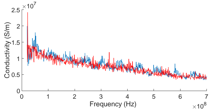
Fig. 3. Conductivity of 200nm and 500nm ITO layer on 350μm AsGa substrat
