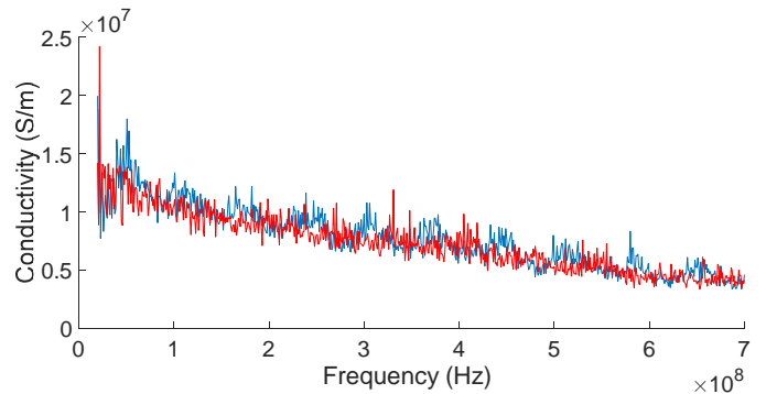
Fig. 3. Conductivity of 200nm and 500nm ITO layer on 350μm AsGa substrat
