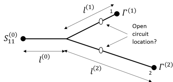
Fig. 1. Location ambiguity of a fault on a complex electrical network topology. Above: Time Domain reflectometer of a Y star-shaped network either adapted at each extremity (—) or affected by an open circuit on a branch (---). Below: The only knowledge of the distance of the fault to the injection point doesn't allow to state on which branch the fault is located.
