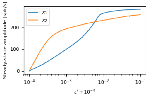
Fig. 2: Steady state amplitude (\max\{x_i(t)\} - \min\{x_i(t)\}) for t \in [19, 20] s for different values of \varepsilon' := \varepsilon T . The remaining parameters were kept identical as in the simulation performed to obtain Figure 1 but with u = 0 . The results obtained are in accordance with Theorem 4 which states that the steady-state amplitude of the system is upper bounded by a \mathcal{K}_\infty class function of \varepsilon + \|u\| . The x-axis is shifted by 10^{-4} to allow displaying values for \varepsilon' = 0 .
