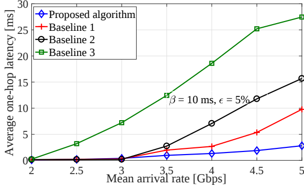
Fig. 3: Average one-hop delay versus mean arrival rates, \epsilon = 5\% , \beta = 10 ms, \kappa = 5 .
