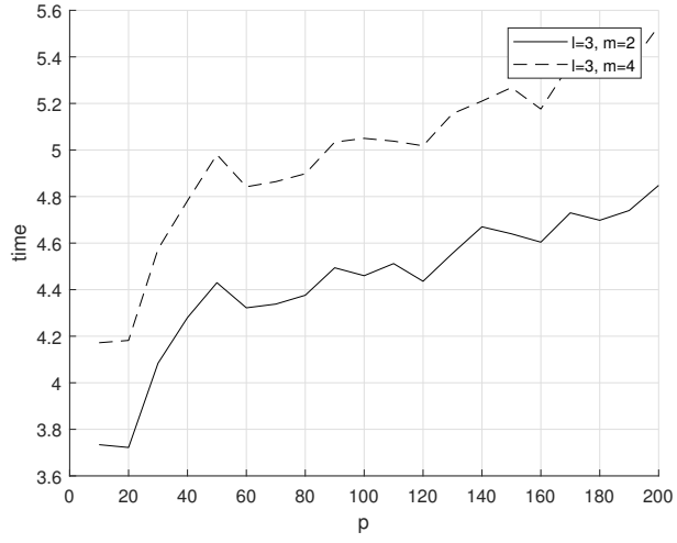
Figure 1: Parallel CY method with GA implementation
