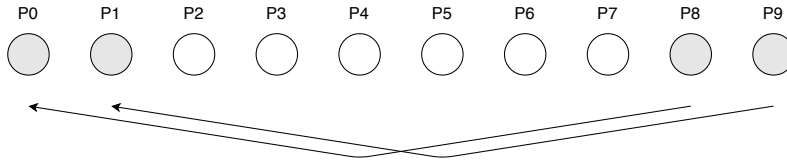
Figure 1: Backward shift
