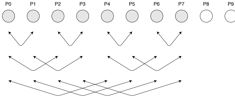
Figure 2: Recursive doubling
