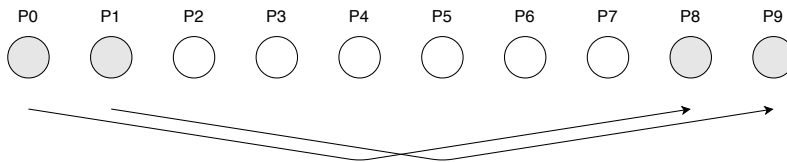
Figure 3: Forward shift
