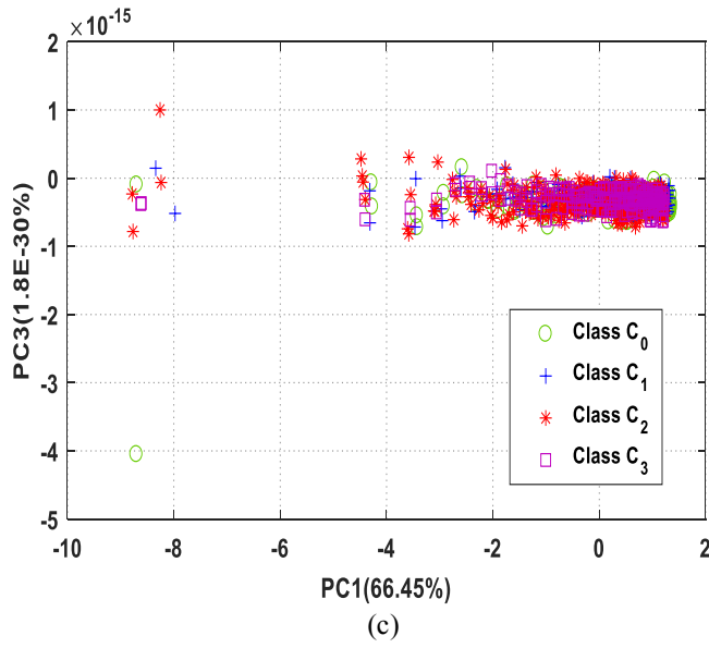
Fig. 8: PCA training data set results in the subspace spanned by PC1 and PC2 (a), PC2 and PC3 (b), PC1 and PC3 (c), and 3D PCA plot
