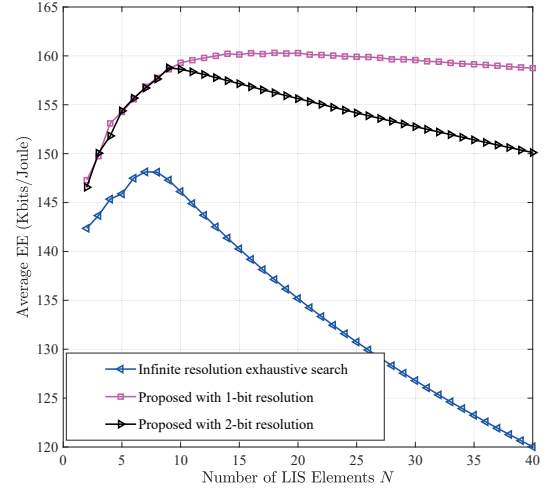
Figure 4. Energy efficiency maximization vs the number of LIS elements N for K = 8 , M = 6 , P_n(2) = 5 dBm, P_n(4) = 15 dBm, P_n(+\infty) = 45 dBm, and R_{\min,k} = 0 bps/Hz \forall k = 1, 2, \dots, 8 .
