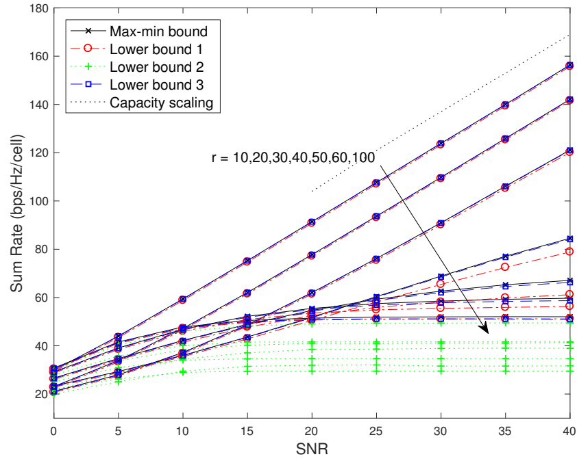
Fig. 3. The impact of spatial despreading on sum-rate scaling of MIMO uplink with respect to the sparsity of angular support ( r ), where M = 200, L = 4, K = 10, T_c = 500 . The max-min bound is given by (29). While ‘Lower bound 1’ is the coherent bound in (24), ‘Lower bound 2’ and ‘Lower bound 3’ indicate the noncoherent ones in (27) and (30), respectively. While r = 100, 60, 10, 20, 50, 30, 40 from top to bottom for Lower bound 2, r = 10, 20, 30, 40, 50, 60, 100 for the rest. The asymptotic capacity scaling is given by (25) with o(1) = 0 .
