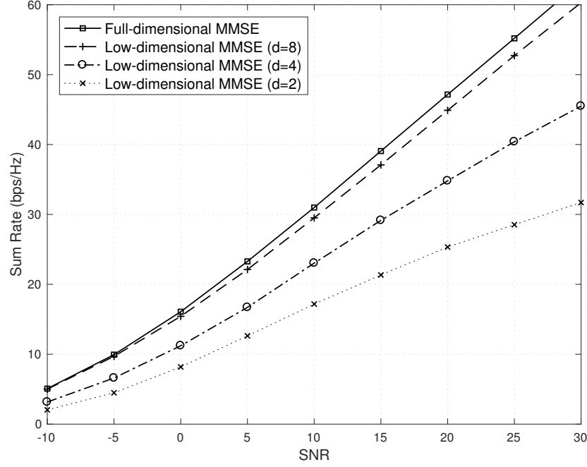
Fig. 2. Sum-rate curves of different precoding schemes versus SNR (dB) in MIMO downlink, where M = 100, L = 4, K = 5, r = 8, T_c = 500 . The random partial Fourier model in (7) was used for channel covariance matrices. For low-dimensional MMSE precoding, we used (23).
