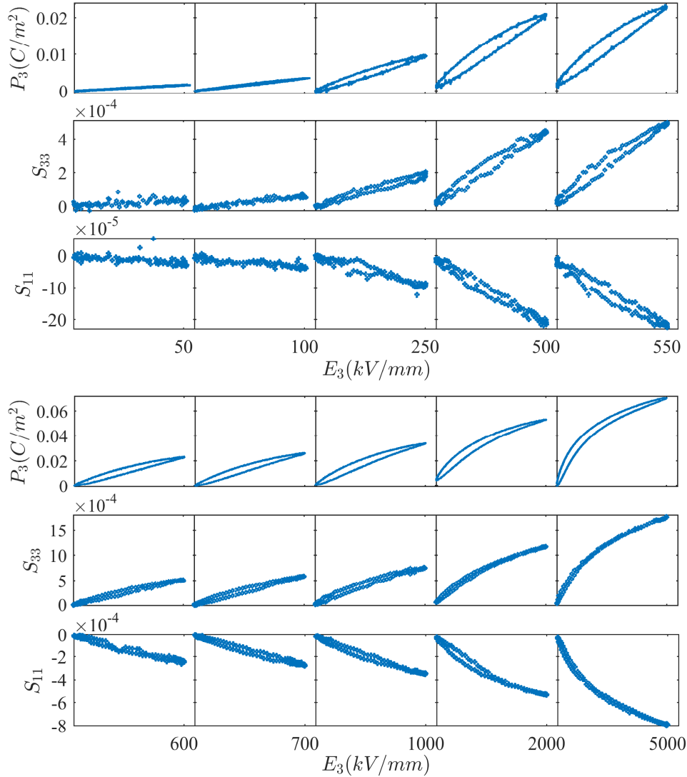
Figure 7 – Polarisation P_3 , longitudinal strain S_{33} and transverse strain S_{11} under growing unipolar sinusoidal electric field (50 mHz). Before measurements, the sample (NCE55) was initially poled at 4000 V/mm during 1 min.
