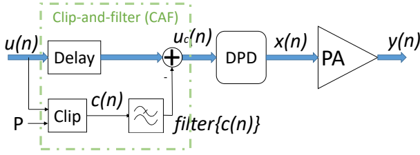
Fig. 1. The structure of CAF in front of DPD.
