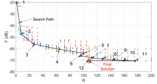
Fig. 4. Search path of New OH-based method ( d=50 )
