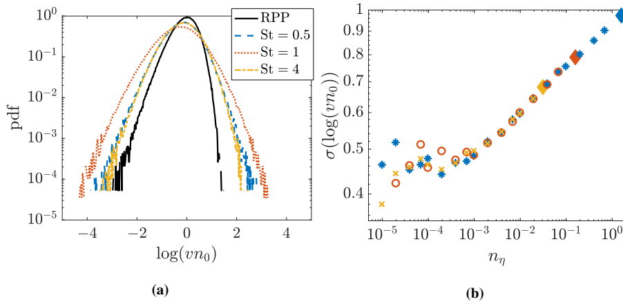
Figure 4: (a) PDF of normalized Voronoi volumes. (b) Evolution of the standard deviation of the PDF with the number of particles in simulations, for successive depletion in post-processing.
