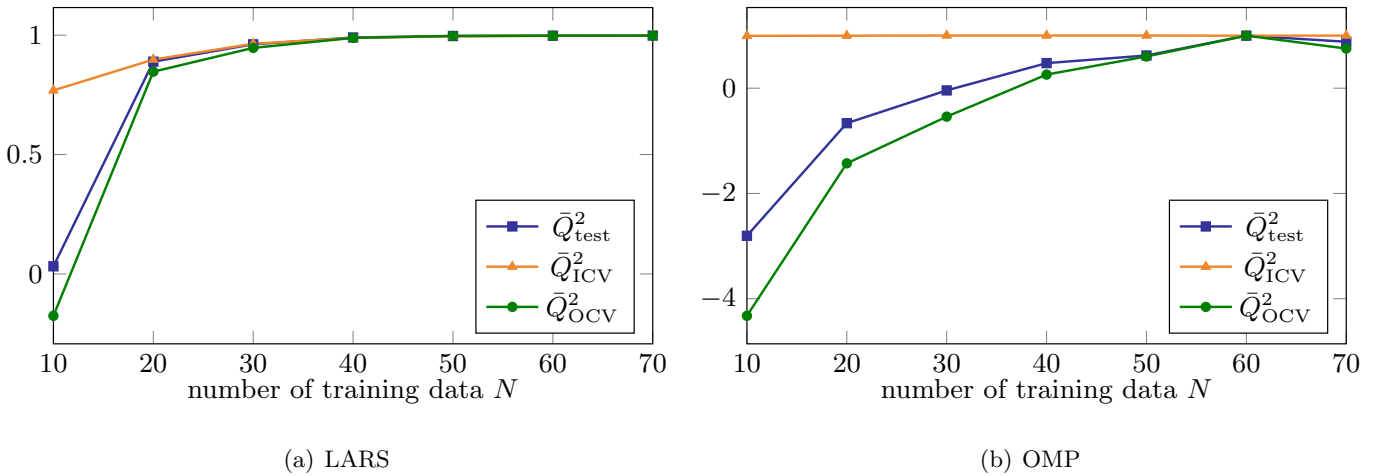
Figure 4: Borehole function - mean of \bar{Q}^2 over 100 replications versus the increasing number of training data.
