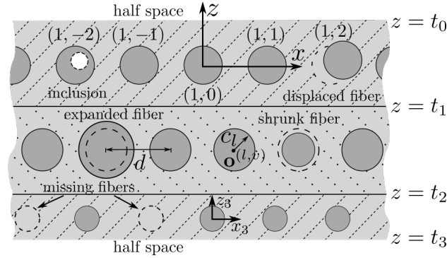
Fig. 1. Sketch of the damaged laminate with defects of concern, L = 3 .
