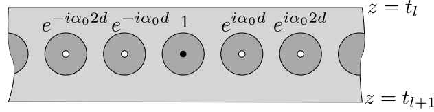
Fig. 5. Phased line-source array, solid dot standing for the true source and hollow ones for fictitious sources.
