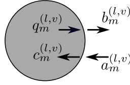
Fig. 3. Field representation by cylindrical-wave expansions in the (l, v) -th fiber.
