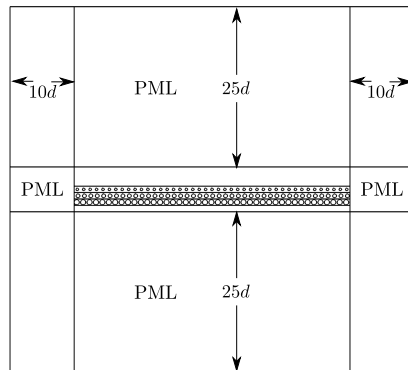
Fig. 8. Geometry of COMSOL module, 43 fibers in each layer of the laminate, fiber radius c_1 = 0.2d , c_2 = 0.3d , c_3 = 0.4d .
