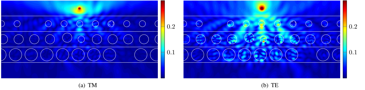
Fig. 11. Amplitude of total (a) electric field and (b) magnetic field with a line-source illumination, \mathbf{r}_s = (0, d) , \lambda^{inc} = d , white lines indicating the laminate structure.
