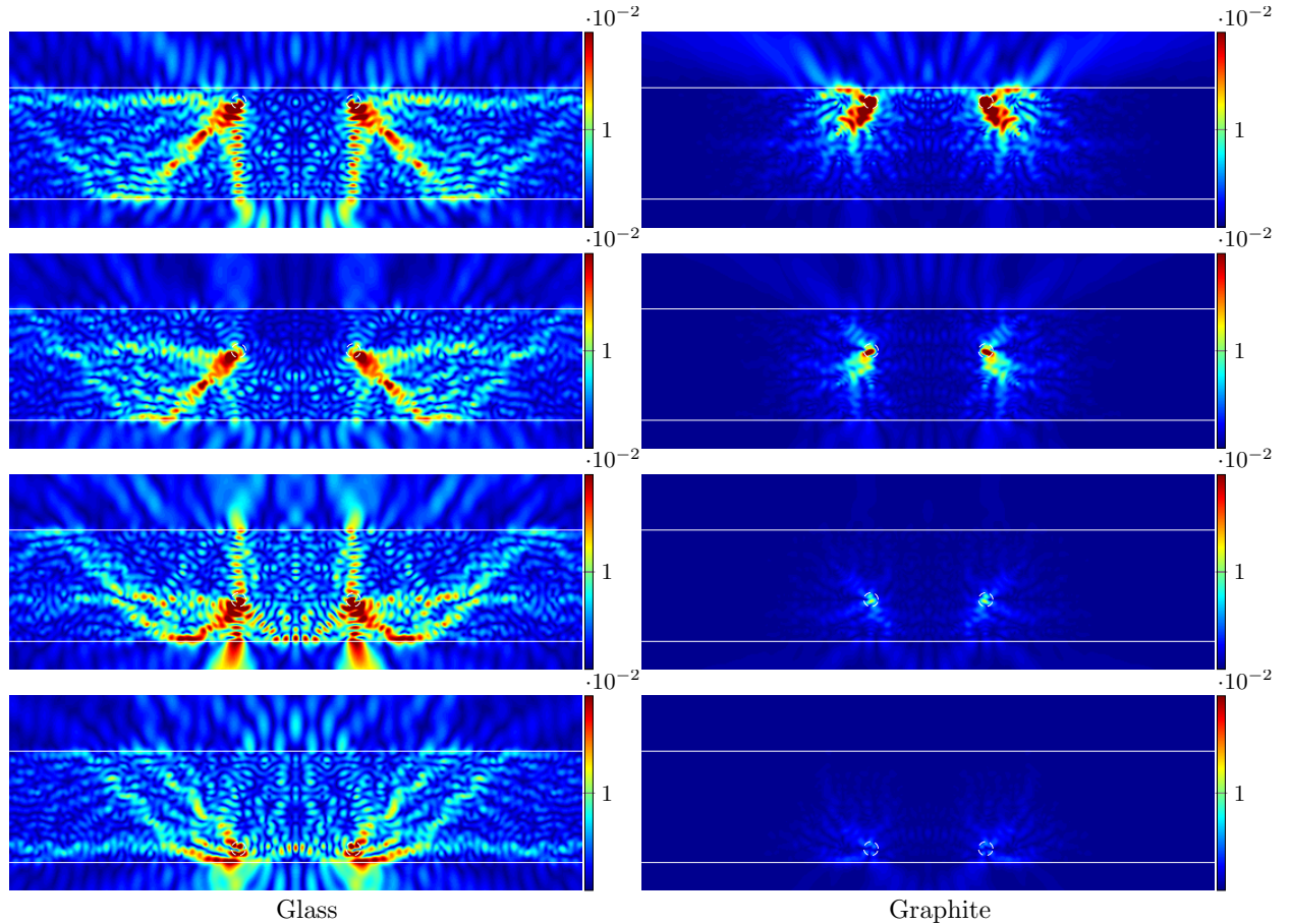
Fig. 14. Maps of anomalous field with the (l, 2) -th and (l, 2) -th fibers missing, l = 1, 2, 3, 4 , line source at (0, d) , \lambda^{inc} = d , TM.
