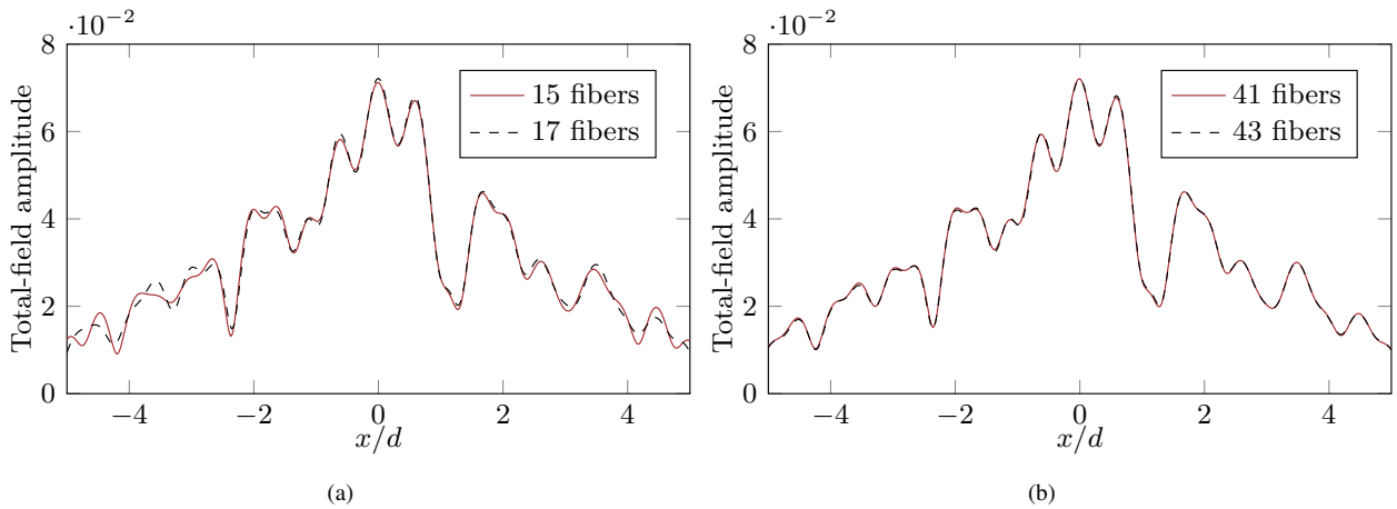
Fig. 9. Amplitude of sampled total fields vs number of fibers in COMSOL, \mathbf{r}_s = (0, 0) , \lambda^{inc} = d , z = d , TM polarization.
