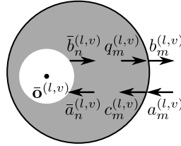
Fig. 6. CWE coefficients inside the fiber with an circular inclusion.
