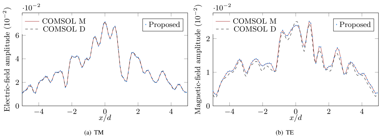
Fig. 10. Validation of the computation of the Green's function by comparisons with COMSOL, \mathbf{r}_s = (0, 0) , \lambda^{inc} = d , z = d , “COMSOL D” denoting COMSOL solution with the default mesh settings and “COMSOL M” with manual settings.
