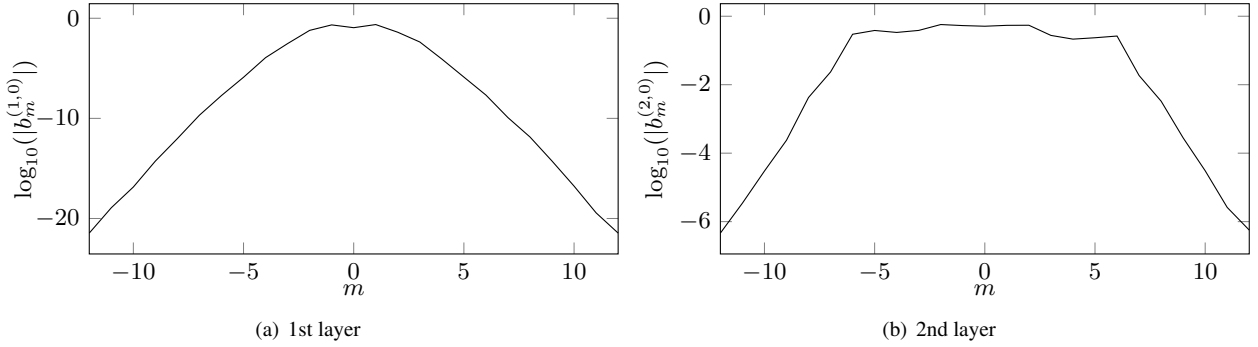
Fig. 7. Line graphs of CWE coefficients b_m , M = 12 , two-layer laminate with the plane-wave illumination, \theta^{inc} = \pi/6 , \lambda^{inc} = d .
