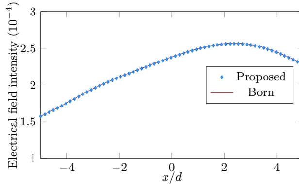
Fig. 13. Anomalous field computed by the proposed approach and the Born approximation, the (1, -3)-th and (3, 3)-th fibers are missing, \mathbf{r}_s = (0, d) , \lambda^{inc} = 100d , TM, z = 1.5d .
