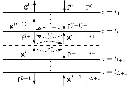
Fig. 4. Equivalence of fiber arrays as planar boundaries with scattering matrices \mathcal{E}_l^u and \mathcal{F}_l^u , u = 1, 2, 3, 4 , defined by Eq. (2) and (11).
