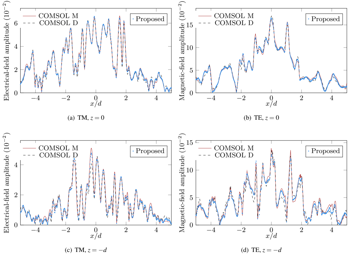
Fig. 12. Validation of modeling the damaged laminate through comparisons with COMSOL, \mathbf{r}_s = (0, d) , \lambda^{inc} = d , “COMSOL D” denoting COMSOL solution with the default mesh settings and “COMSOL M” with manual settings.
