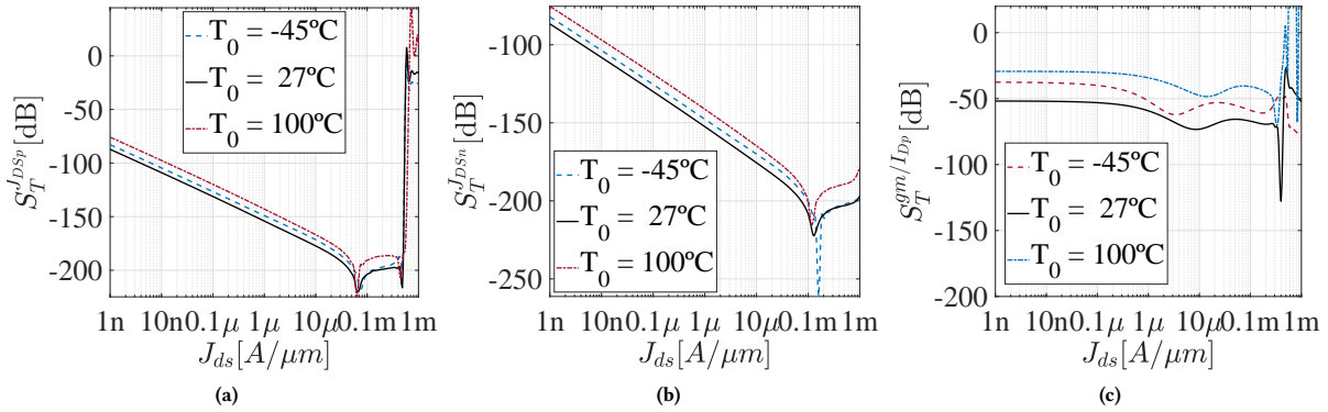
Figure 3: Ideal Wilson current mirror is used for parameters extraction: (a) S_T^{Dsp} (b) S_T^{Dsn} (c) S_T^{gmp/IDp}
