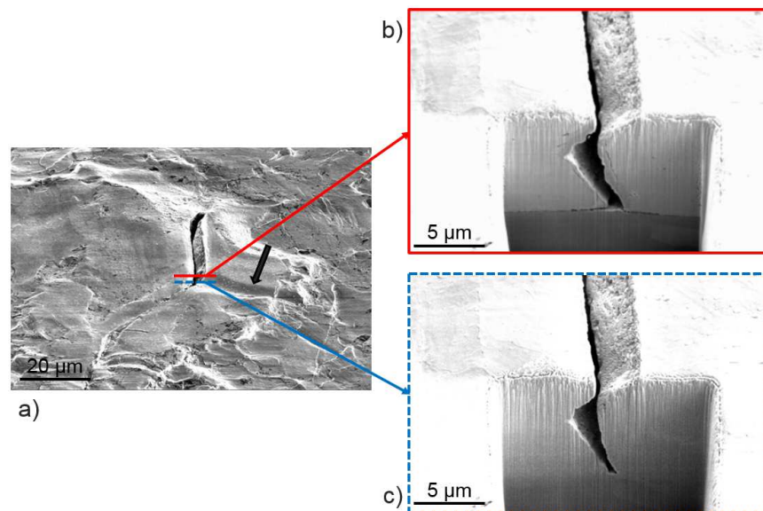
Figure 12 – Crack between two zinc grains on a plateau (note the presence of a trace of dendrite noted by the arrow in Figure a). a) BSE surface observation after 0.12 strain; b) and c) in-depth view of the cracks at two different locations along the grain boundary after FIB machining.
