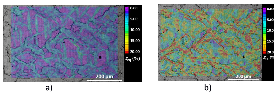
Figure 8 – Local equivalent strain of zinc coating on a 300 \times 300 \mu\text{m}^2 area for an average strain equal to 2% (a) and 11% (b).
