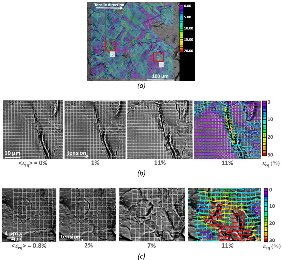
Figure 9 – Surface damage evolution during in situ straining.
