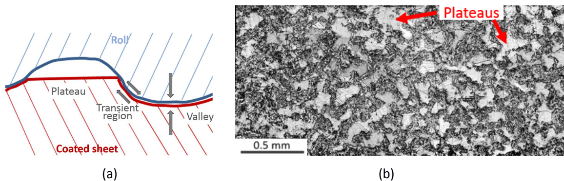
Figure 2 – (a) A schematic description of roughness transfer from roll to sheet surface: valleys are mostly submitted to plane compression, and transient regions to shear; (b) EBSD Band Contrast map of the coating surface after temper rolling: the non-deformed plateaus appear as smooth light grey areas.
