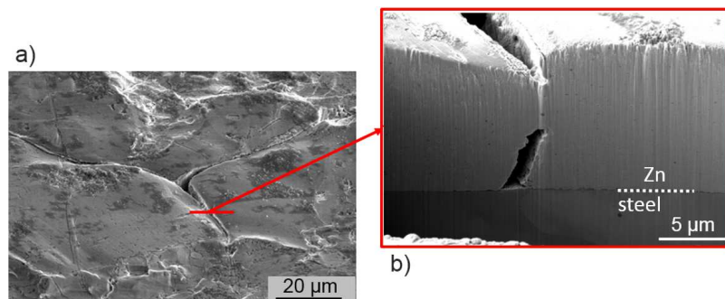
Figure 11 – Crack at a triple point junction on a plateau. a) BSE surface observation after 0.12 strain; b) in-depth view of the crack after FIB machining.
