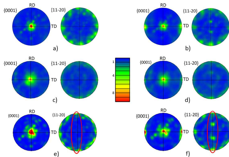
Figure 7 – \{0001\} and \{11-20\} pole figures of zinc grains calculated from 3 \times 3 \text{ mm}^2 EBSD maps after temper rolling along RD (a, c, and e) and after 0.12 tensile strain along TD (b, d, and f).
