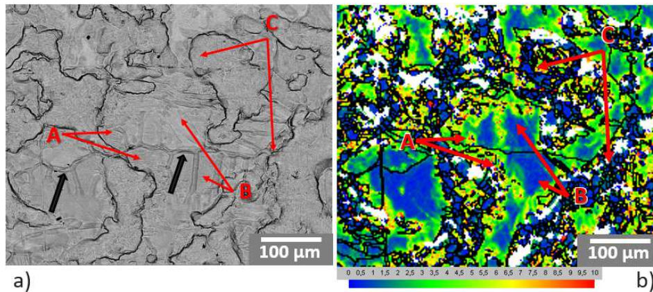
Figure 3 – Zinc surface after temper rolling: (a) BSE image (traces of solidification dendrites are indicated by black arrows); (b) KAM map of the same area (colors quantify the local misorientation from 0 to 10° according to the bar below the figure, and black lines delineate grain boundaries). A, B, and C denote examples of transient regions, plateaus, and valleys respectively, as sketched in Figure 2.a.
