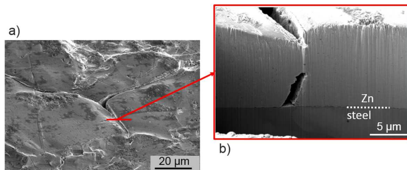
Figure 11 – Crack at a triple point junction on a plateau. a) BSE surface observation after 0.12 strain; b) in-depth view of the crack after FIB machining.
