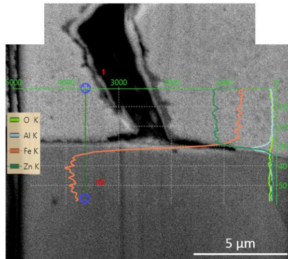
Figure 13 – EDX analysis of the zinc – steel interface after deformation (same cross section as Fig. 12.b).
